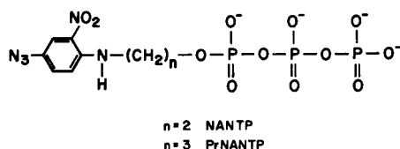
FIGURE 1 Structures of NANTP and PrNANTP.
