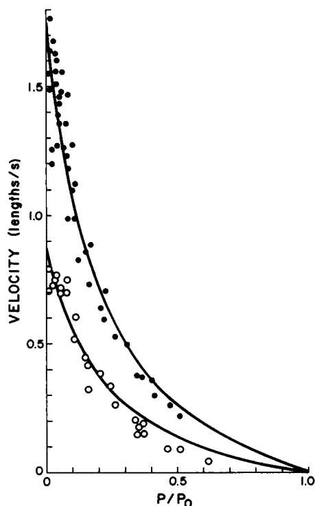
FIGURE 5 Contraction velocity plotted as a function of tension normalized to the isometric value using buffers containing 4 mM MgNANTP and either 4 mM NANDP (O) or 15 mM P_i (●). Solid lines are least-squares Hill fits (Eq. 1) as described in Methods. Values of isometric tensions and maximum shortening velocity are given in Table 3.
