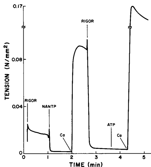
FIGURE 2 Tension as a function of time for a fiber activated first in MgNANTP and subsequently in MgATP. The fiber was first washed in a nucleotide-free rigor buffer, then relaxed in a buffer containing 4 mM MgNANTP. After activation by addition of Ca^{2+} , an isometric tension of 0.09 N/mm 2 was obtained. MgNANTP was subsequently washed out using rigor buffer. Immersion in buffer containing 4 mM MgATP relaxed the fiber. After addition of Ca^{2+} , normal isometric tension of 0.17 N/mm 2 was obtained. Solution changes/additions were as noted.
