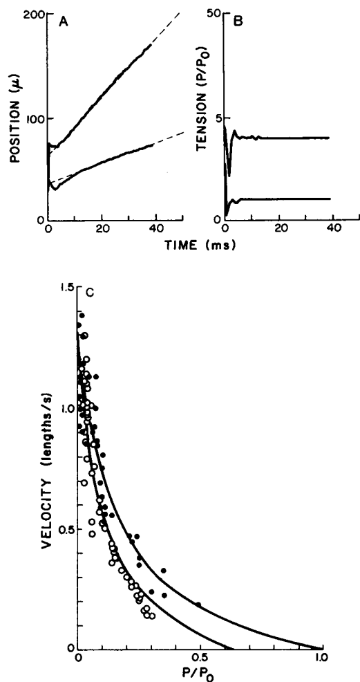
FIGURE 3 (A) Length and (B) tension of a single fiber as a function of time for a series of two isotonic releases. Traces in A show the position of the motor arm attached to the fiber. The dashed lines are least-squares fits to position data taken over the period 10–40 ms. Traces in B show tension as a function of time, normalized to isometric tension. The displacement trace with the greater slope (velocity) corresponds to the lower release tension. The fiber was activated and the two isotonic releases were made within 20 s. After release, the fiber was reextended at a velocity of 1 mm/s. Traces from a single fiber, length = 3.1 mm, 4 mM MgNANTP. (C) Shortening velocity plotted as a function of tension for 4 mM MgATP (●) and 4 mM MgNANTP (○) from a series of experiments as in A and B. Solid lines are least-squares Hill fits (Eq. 1) as described in Methods. Tensions are normalized with respect to the isometric value at 4 mM MgATP.
