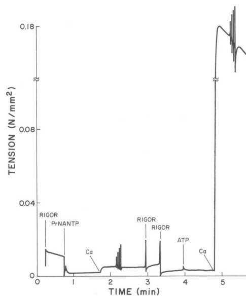
FIGURE 4 Tension as a function of time for a fiber activated first in MgPrNANTP and subsequently in MgATP. The fiber was first washed in a nucleotide-free rigor buffer, then relaxed by addition of 4 mM MgPrNANTP. After activation by addition of Ca 2+ , no rise in isometric tension was obtained. The transient deviations in the plot were attempts at isotonic releases. MgPrNANTP was subsequently washed out by exchanging the solution for rigor buffer. Addition of 4 mM MgATP relaxed the fiber. After addition of Ca 2+ , normal isometric tension of 0.16 N/mm 2 was obtained, with subsequent transients showing normal shortening velocities of 0.8, 1.0, and 1.2 muscle lengths/s for isotonic releases of 10, 5, and 1% P_o , respectively. Solution changes/additions were as noted.
